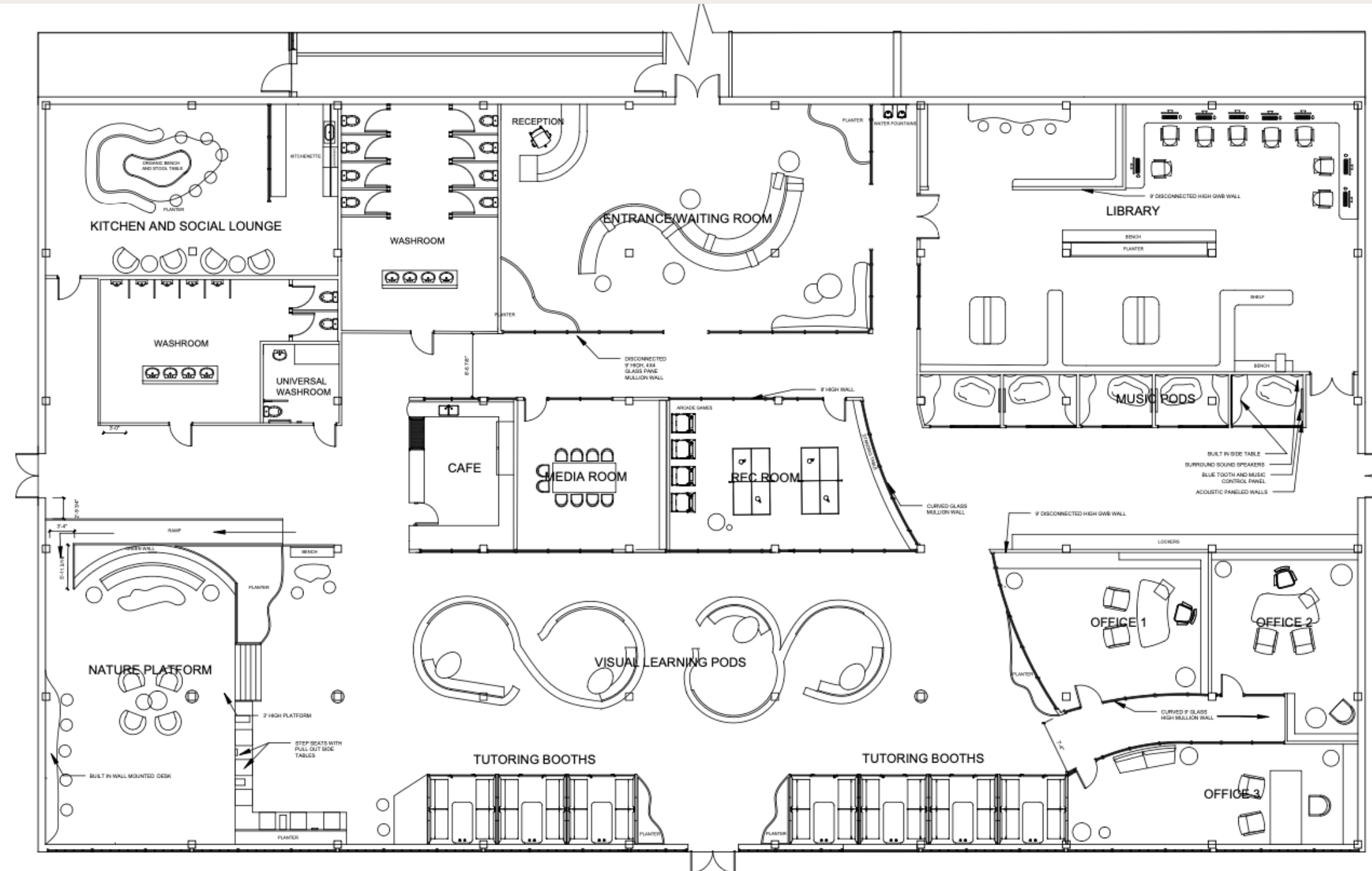
2 DEVELOPED FLOOR PLAN ID-2 SCALE : 1/8"=1'-0"
